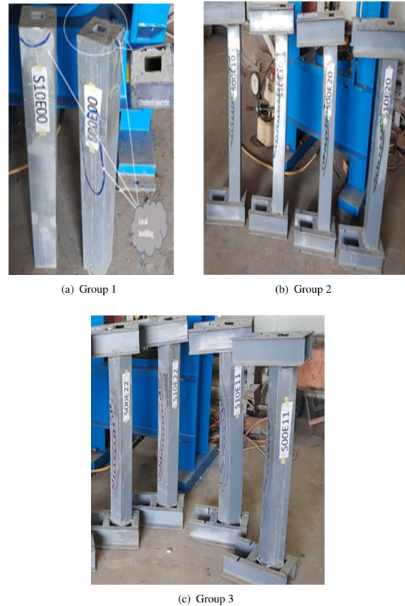
Figure 4. Failure modes.
