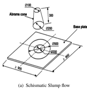
(a) Schematic Slump flow
