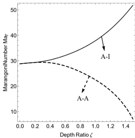
Figure 2. Comparison of Adiabatic–Adiabatic and Adiabatic–Isothermal boundary conditions.
