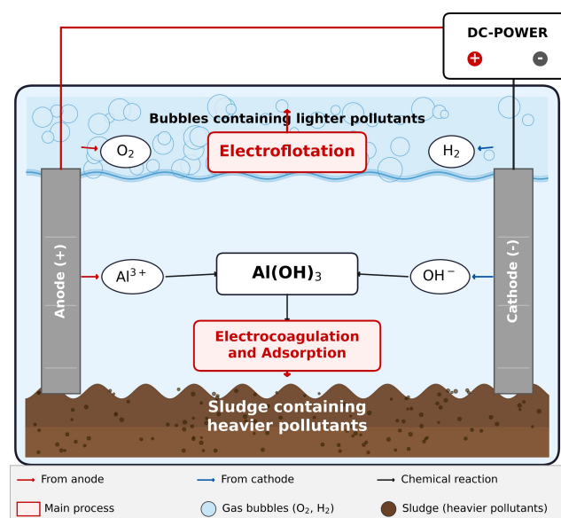
Figure 15. The mechanism suggested for AC – EC treatment.
