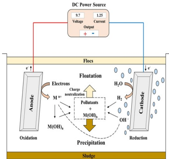
Figure 1. The electrocoagulation Mechanism [16].
