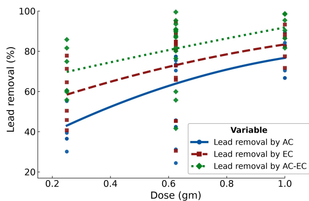
Figure 10. Effect of dose on the lead removal.
