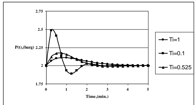
Figure (4) Experimental system response of PI-controller to step change in inlet pressure (P 1 ) at K C = 5 with different τ I (min.).
