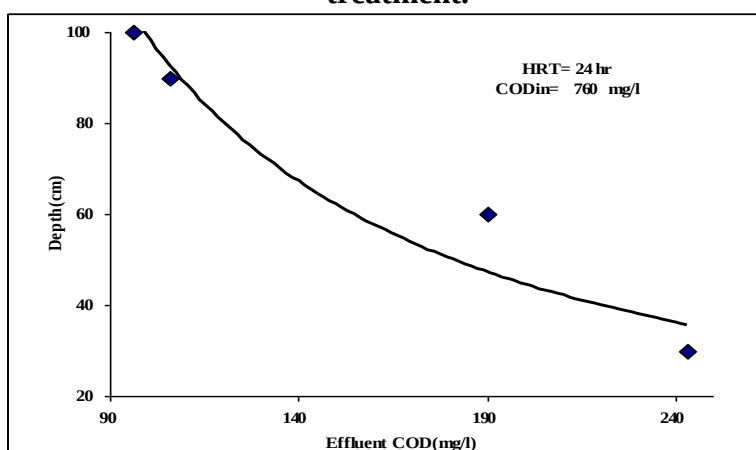
Fig (4) The Effluent COD with the depth of filter(1 st run)-anaerobic treatment.
