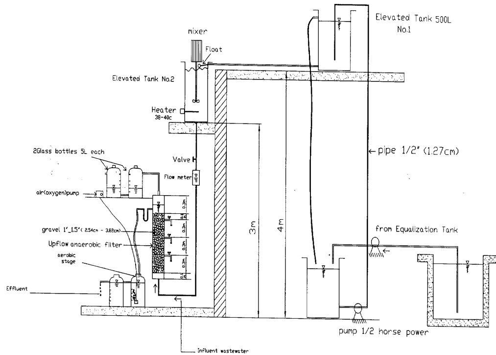
Fig (1) Schematic diagram of the pilot plant.
