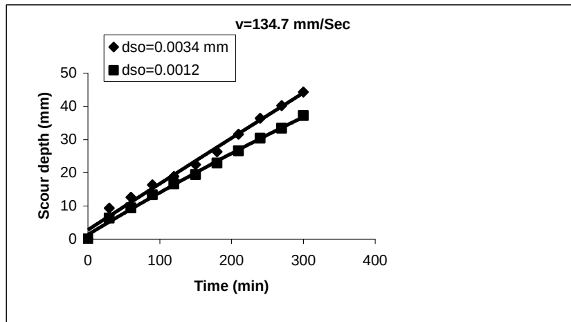
Fig(4) Scour depth versus time in clay bed material .
