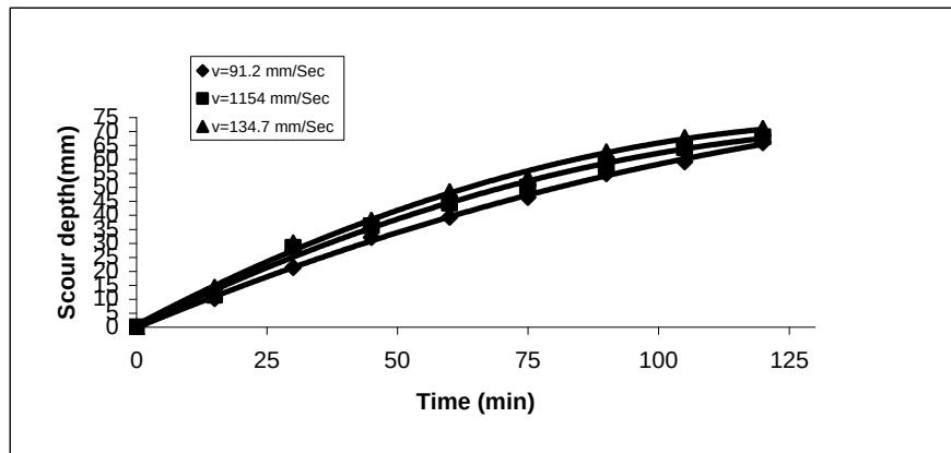
Fig(2) Measured scour depth versus time in sand bed material ( d_{50}=0.45 mm)
