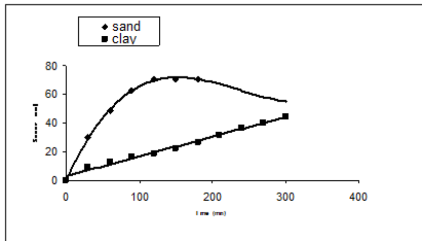
Fig . (5). Comparison of scour depth between sand and clay beds
