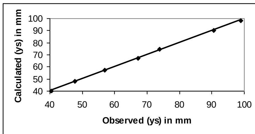
Fig . (8) : Calculated scour depth versus observed scour depth in sand soil
