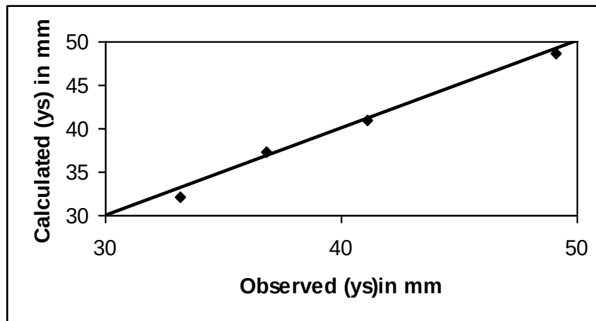
Fig. (7): Calculated scour depth versus observed scour depth in clay soil.
