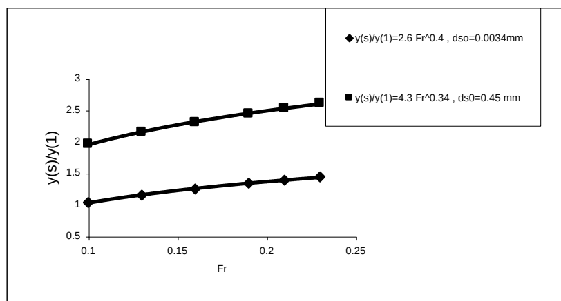
Fig (6) Variations in relative scour depth with Froude number
