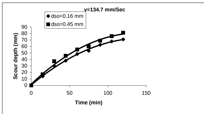
Fig(3) Scour depth versus time in sand bed material .
