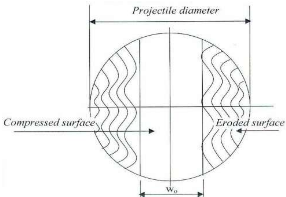
Fig.(6): Schematic of a photograph of damage surface of cylindrically-convex Aluminum plates produced by a flat-ended wax projectile.
