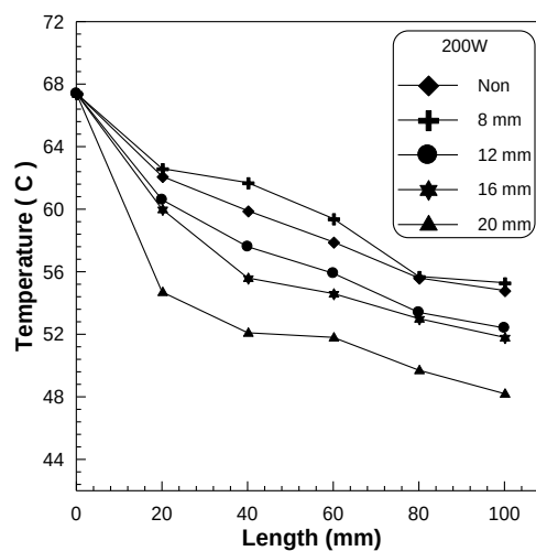
Figure (6) Temperature Distribution with 200w
