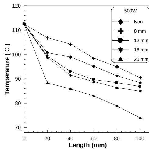
Figure (9) Temperature Distribution with 500w
