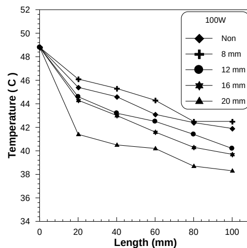
Figure (5) Temperature Distribution with 100w
