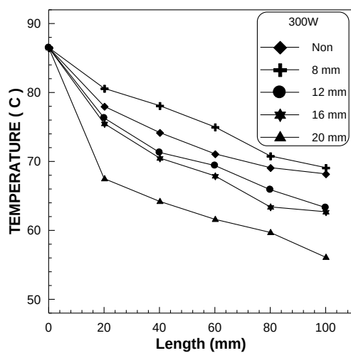
Figure (7) Temperature Distribution with 300w
