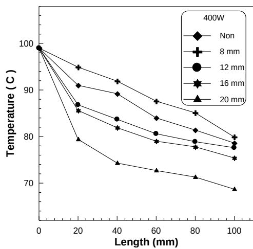
Figure (8) Temperature Distribution with 400w
