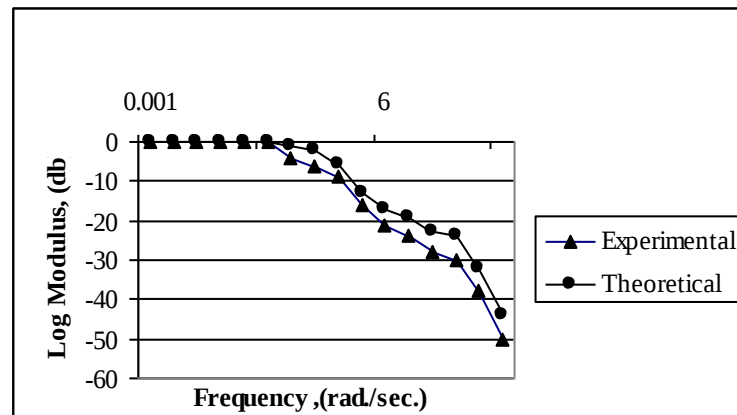
Figure (4) Bode plot of heat exchanger (log modulus) at flow rate 5 lit./min. and duration equal to 120 sec.
