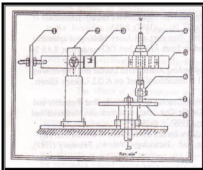
Fig.1. Schematic drawing of the pin on disc sliding machine.
