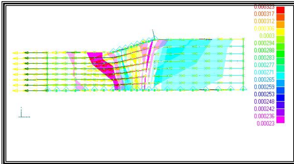
Fig. (9). major strain distribution when R=25%, friction Factor=0.1, semi die angle = 15°.
