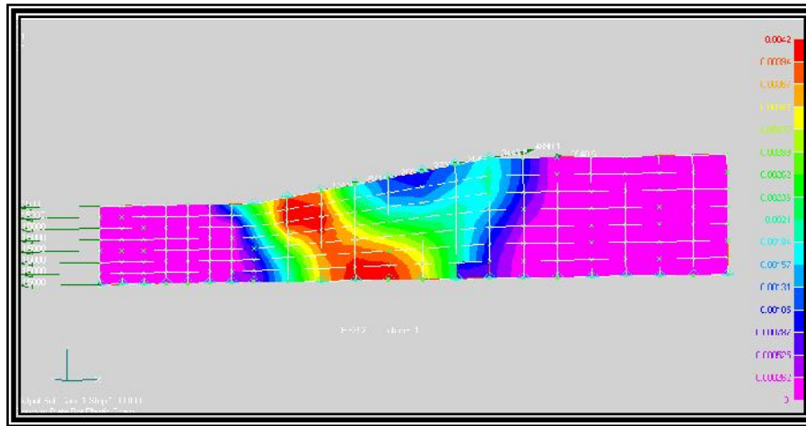
Fig. (8). major strain distribution when R=35% & friction Factor=0.1, semi die angle = 15°
