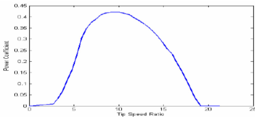
Fig. (1-b): Power Coefficient Verses Tip Speed Ratio.
