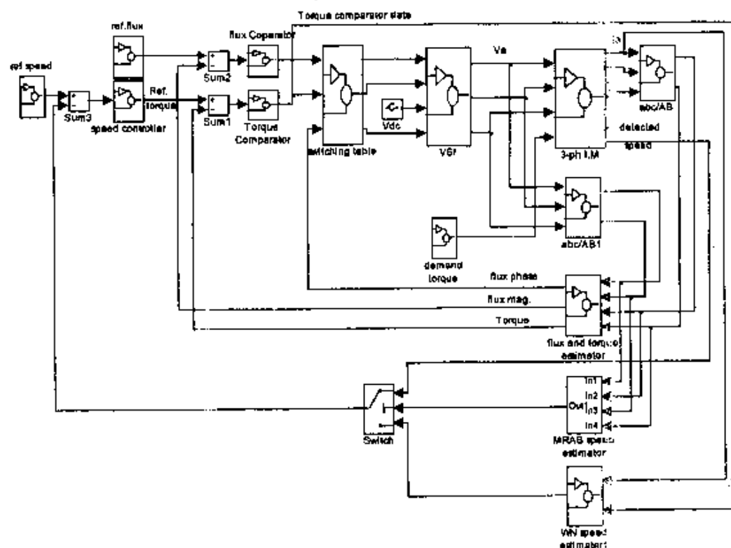
Fig. (5) Mathlap simulink block diagram for DTC induction motor drive.
