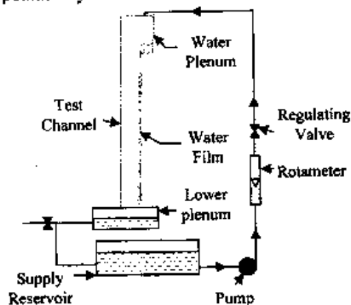
Figure (1) Schematic Diagram of the Experimental Apparatus
