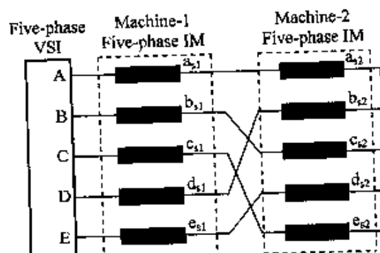
Fig.1 Five-phase series-connected two-motor drive system.
