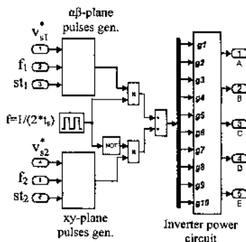
Fig.6 The whole Simulink model of the VSI supply system.
