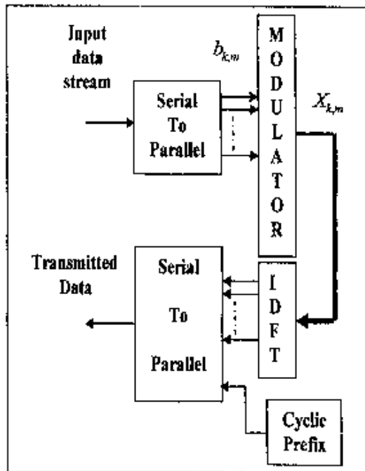
Figure 1: Digital multi-carrier transmission system applying OFDM.
