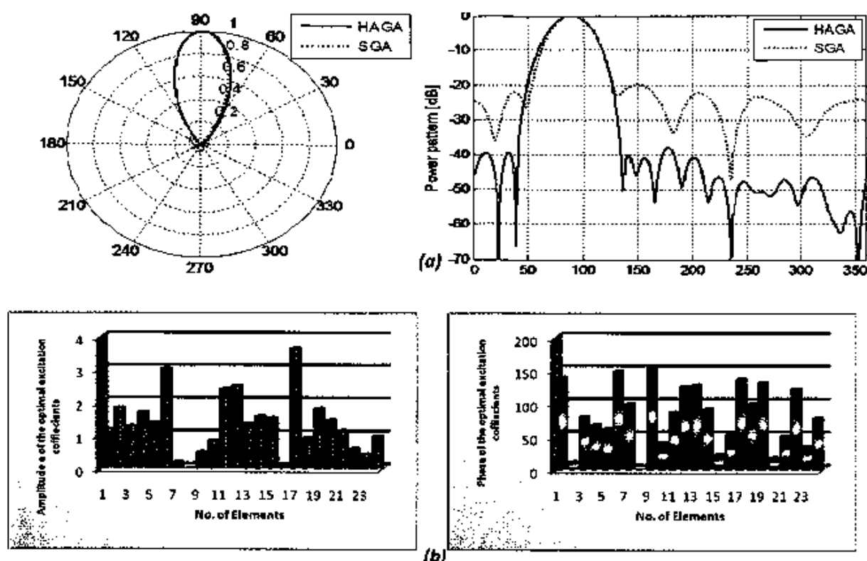
Figure 4: (a) plots of the optimized radiation patterns; (b) plots of elements' excitation coefficients of the optimized circular array antenna with 25 elements
