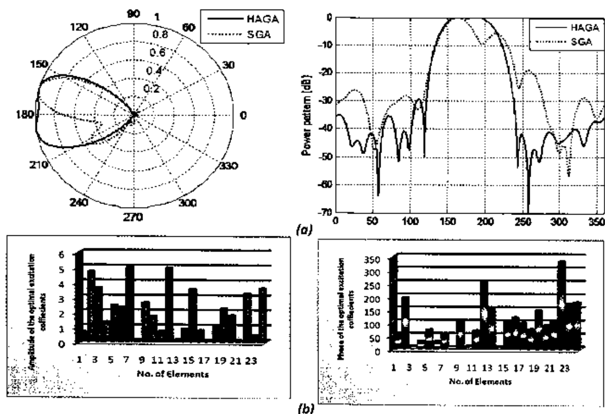
Figure 5: (a) plot of the optimized radiation pattern with wide flat main beam extends from \phi=150^\circ to \phi=210^\circ ; (b) the plots of elements' excitation coefficients of the optimized circular array antenna with 25 elements
