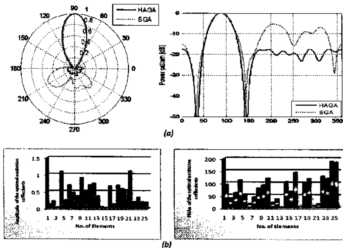
Figure 9: (a) Plots of the optimized Radiation patterns with two imposed broad nulls centered at 35^\circ , 145^\circ with \Delta\phi = 10^\circ ;(b) plots of elements' excitation coefficients
