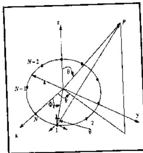
Figure (3): Geometry for a circular array antenna
