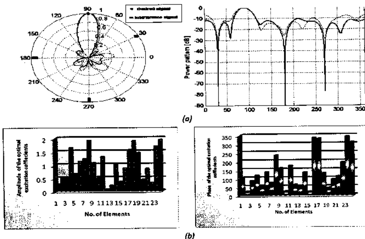
Figure 7: (a) Plots of the optimized pattern with triple imposed nulls at 30^\circ , 180^\circ , and 270^\circ ; (b) the plots of elements' excitation coefficients of the optimized circular array antenna with 25 elements
