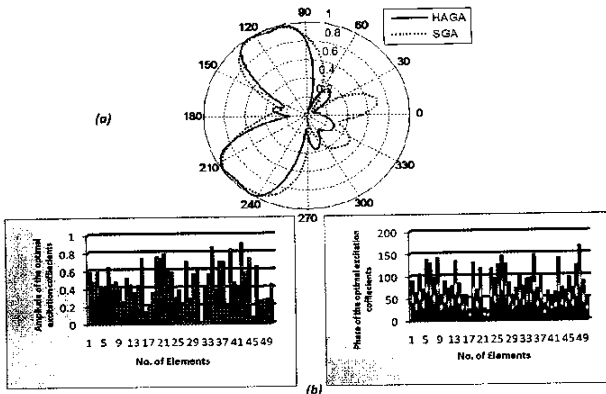
Figure 6: (a) Plot of the optimized radiation pattern with two flat beams; (b) plots of elements' excitation coefficients of the optimized circular array antenna with 50 elements
