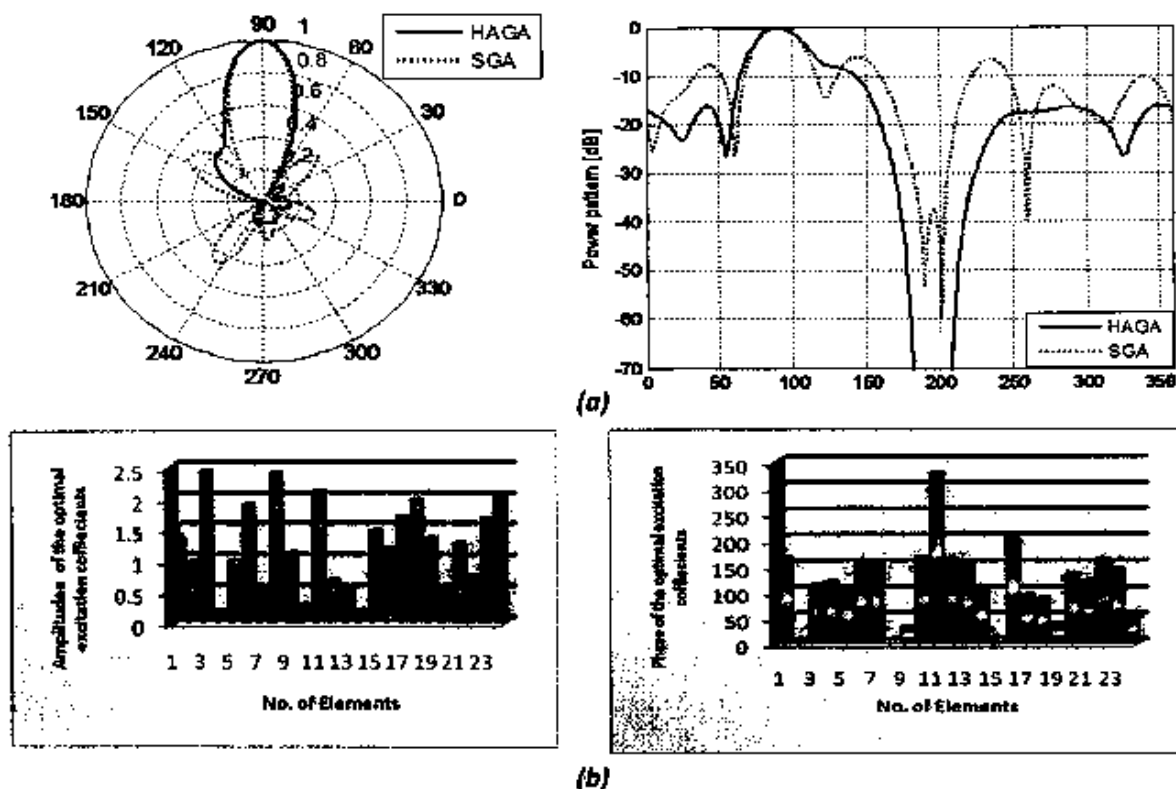
Figure 8: (a) Plots of the optimized radiation patterns with imposed broad null centered at 185^\circ , with \Delta\phi = 30^\circ (b) plots of elements' excitation coefficients of the optimized circular
