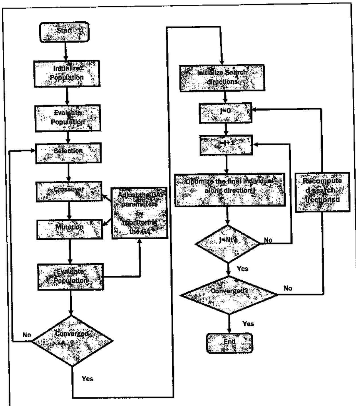
Figure (2): Flowchart of the hybrid adaptive genetic algorithm.
