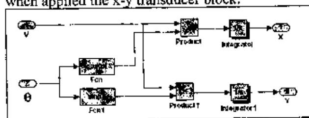
Fig.9: A simulink model of transducer blocks to transfer from velocity and azimuth into ( X_c , Y_c ) coordinates
