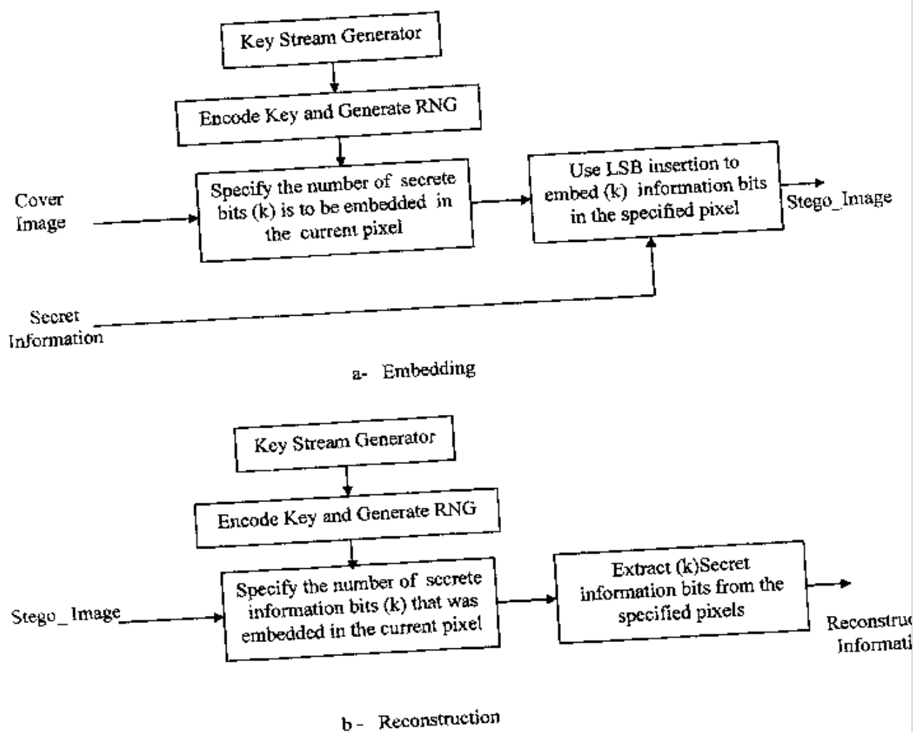
Figure 2: The block diagram of the proposed hiding System
