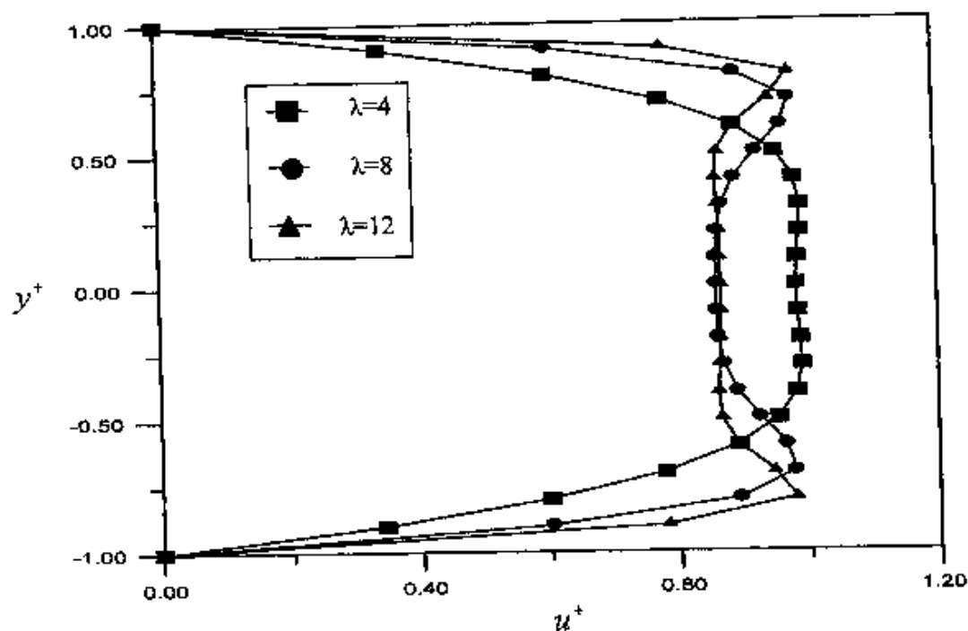
Fig.4 The Effect of Womersley number \lambda on the dimensionless velocity profile at \omega t = 60^\circ , for A_o = 15 , Pr = 0.7 and x / D_h = 20 .
