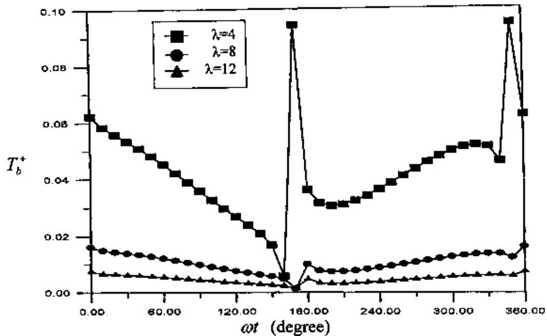
Fig.6 The Effect of Womersley number \lambda on the instantaneous dimensionless bulk temperature at A_o=15 , Pr=0.7 and x/D_h=20 .
