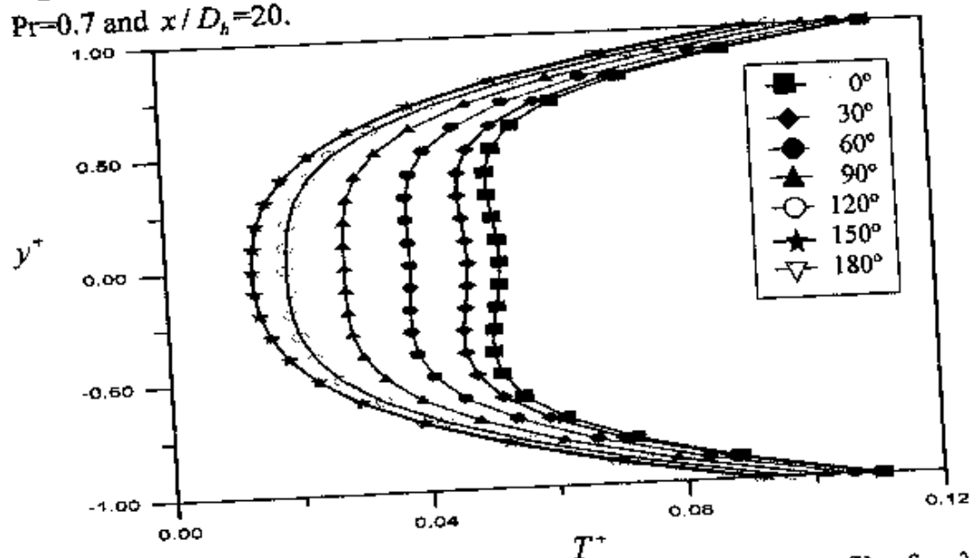
Fig.3 The Variation of the dimensionless temperature profile for \lambda=4 , A_0=15 , Pr=0.7 and x/D_h=20 .
