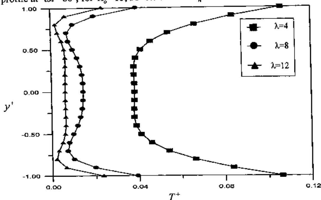
Fig.5 The Effect of Womersley number \lambda on the dimensionless temperature profile at \omega t = 60^\circ , for A_o = 15 , Pr = 0.7 and x / D_h = 20 .
