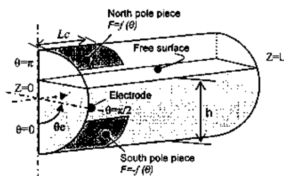
Fig. 3 One-fourth of the original flowmeter volume representing the domain of the numerical solution
