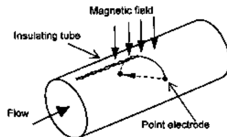
Fig.1 Principle of conventional electromagnetic flowmeter
