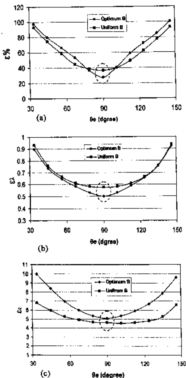
Fig.7 Values of three formulas of \varepsilon 's for two types of magnetic field. The liquid fully fills the flowmeter volume.
