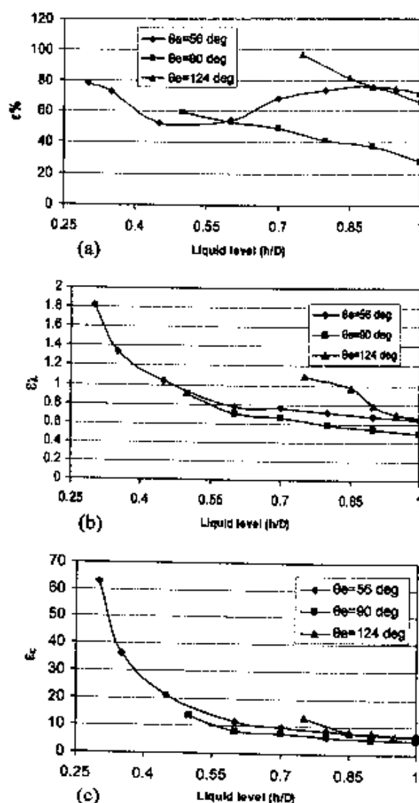
Fig.8 Values of three formulas of \varepsilon 's for optimum magnetic field. The liquid partially fills the flowmeter volume.
