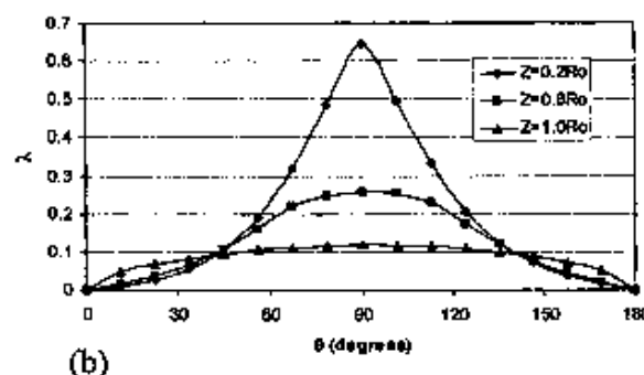
Fig.6 Distribution of \lambda over the flowmeter wall, r=R_o for (a) uniform magnetic field and (b) optimum magnetic field
