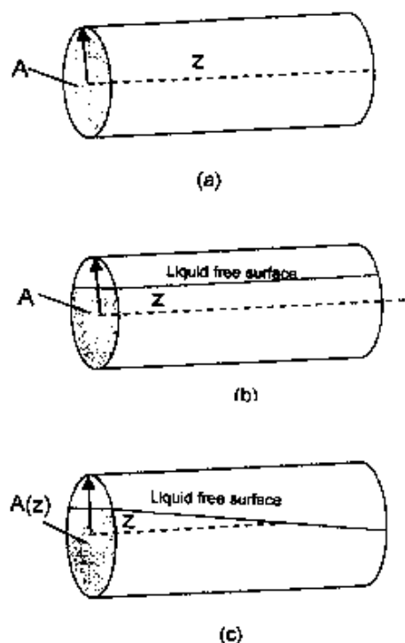
Fig.2 Three types of flow geometry (a) fully filled flow (b) partially filled flow with constant cross- sectional area and (c) partially-filled flow with variable cross sectional area. Z is the axial coordinate.
