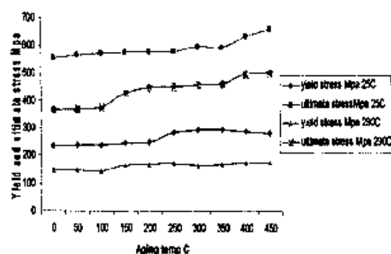
Fig.(7) Show the effect of the aging temperatures on the yield and ultimate stresses at the aging time t=2570 h. for the test temp. T=25^{\circ}\text{C} & T=290^{\circ}\text{C}
