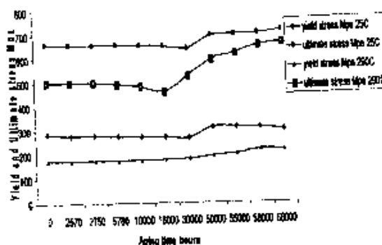
Fig.(19) show the effect of the aging time on the yield and ultimate stress on the aging temperature T=450^{\circ}\text{C} at the test temperature T=25^{\circ}\text{C} and T=290^{\circ}\text{C} .
