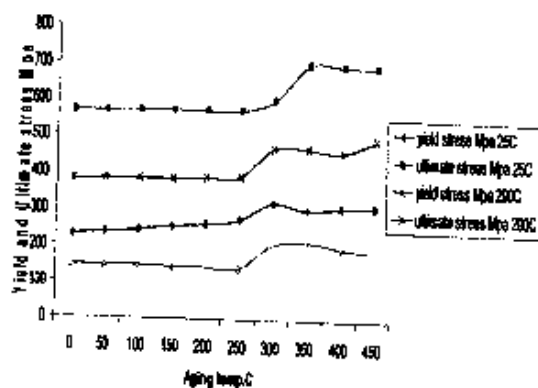
Fig.(11)Show the effect of the aging temperatures on the yield and ultimate stresses at the aging time t=18000 h. for the test temp. T=25^{\circ}\text{C} & T=290^{\circ}\text{C}
