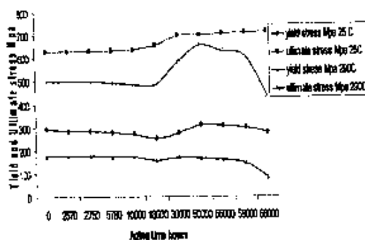
Fig.(18) show the effect of the aging time on the yield and ultimate stress on the aging temperature T=400^{\circ}\text{C} at the test temperature T=25^{\circ}\text{C} and T=290^{\circ}\text{C} .
