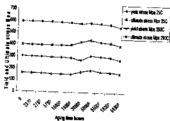
Fig.(15)show the effect of the aging time on the yield and ultimate stress on the aging temperature T=290^{\circ}\text{C} at the test temperature T=25^{\circ}\text{C} and T=290^{\circ}\text{C} .
