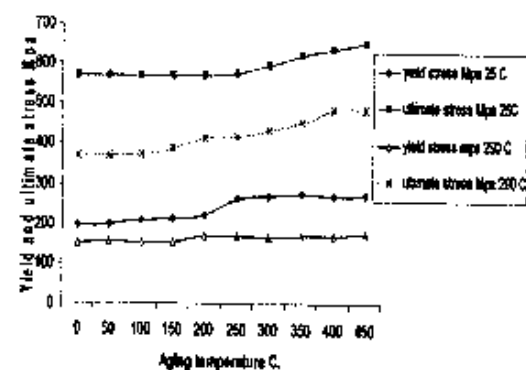
Fig. (6) Show the effect of the aging temperatures on the yield and ultimate stresses at the aging time t=10000 h. for the test temp. T=25^{\circ}\text{C} & T=290^{\circ}\text{C}
