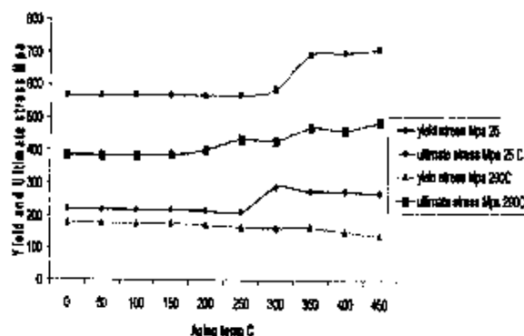
Fig.(8) Show the effect of the aging temperatures on the yield and ultimate stresses at the aging time t=30000 h. for the test temp. T=25^{\circ}\text{C} & T=290^{\circ}\text{C}
