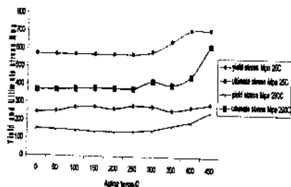
Fig.(13)Show the effect of the aging temperatures on the yield and ultimate stresses at the aging time t=68000 h. for the test temp. T=25^{\circ}\text{C} & T=290^{\circ}\text{C}
