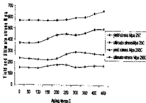
Fig.(9) Show the effect of the aging temperatures on the yield and ultimate stresses at the aging time t=5780 h. for the test temp. T=25^{\circ}\text{C} & T=290^{\circ}\text{C}
