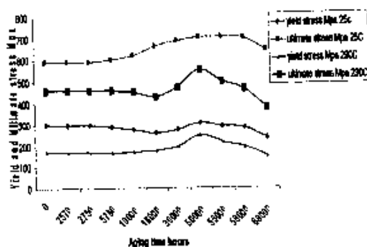
Fig.(17) show the effect of the aging time on the yield and ultimate stress on the aging temperature T=350^{\circ}\text{C} at the test temperature T=25^{\circ}\text{C} and T=290^{\circ}\text{C} .
