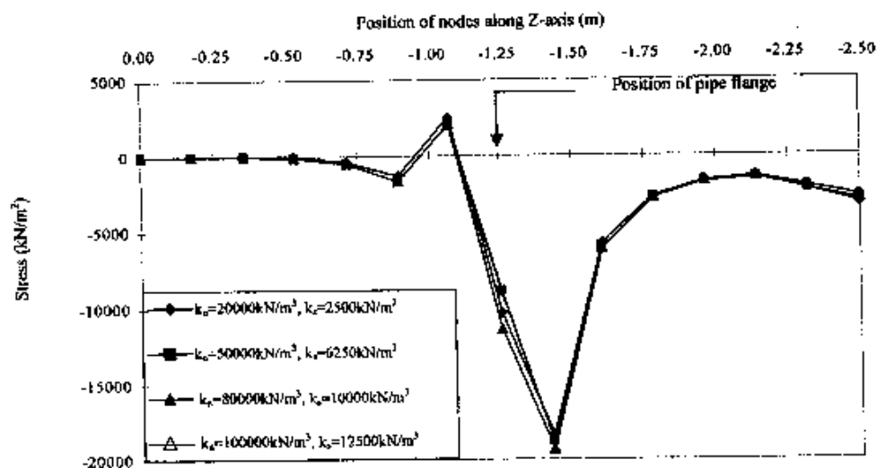
Fig. (7): Stresses-Position of Nodes along the Z-Axis for Model 1, at Top of Pipe.
