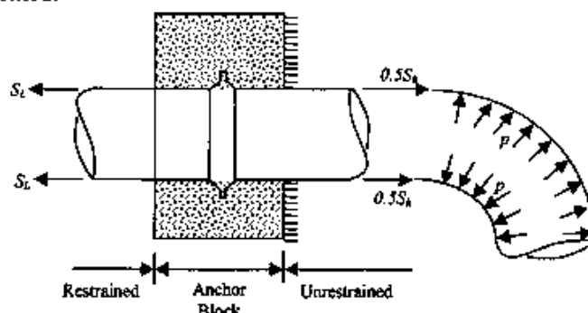
Fig. (1): Anchor Force, from Anchor Installed to Limit Movement of Pipe. [3]
