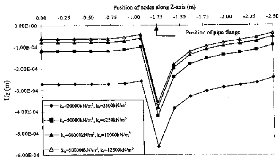
Fig. (9): U_z -Deformations of Nodes along Z-Axis at Top of Pipe.
