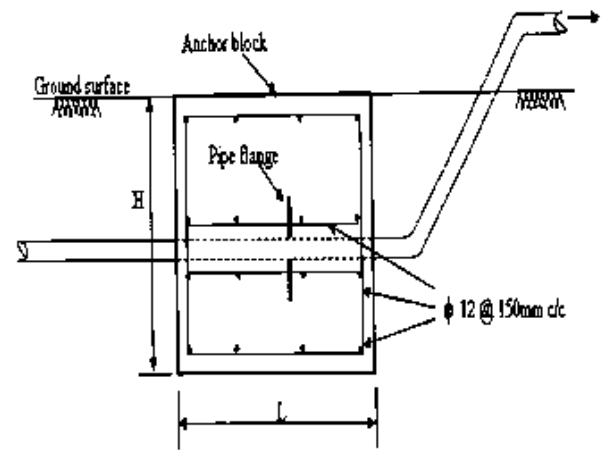
b- A Typical Section of Anchor Block with Reinforcement.
