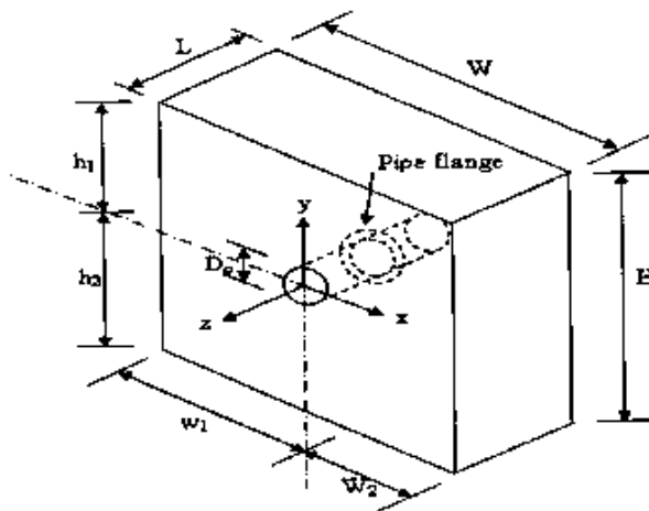
a- Dimensions of Anchor Block.
