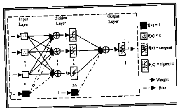
Figure 6: Schematic Diagram of the NN Architecture
