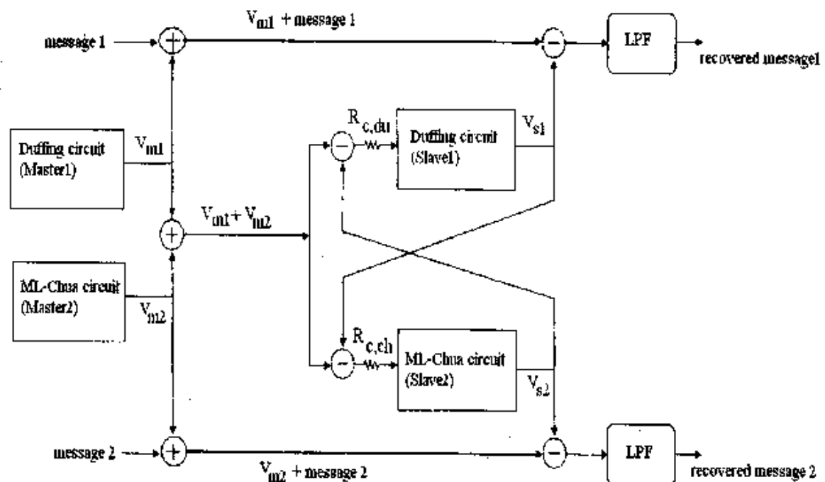
Figure 7. Block diagram of communication scheme (CMS) based on dual synchronization of chaos.
