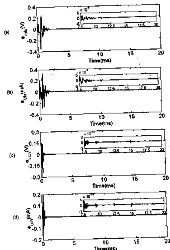
Figure 5. Temporal waveform of the error in the pair of Duffing circuits ((a) and (b)) and in the pair of ML-Chua circuits ((c) and (d)). e_{v,du} = V_{c,m1} - V_{c,s1} , e_{i,du} = I_{L,m1} - I_{L,s1} , e_{v,ch} = V_{c,m2} - V_{c,s2} , and e_{i,ch} = I_{L,m2} - I_{L,s2} .
