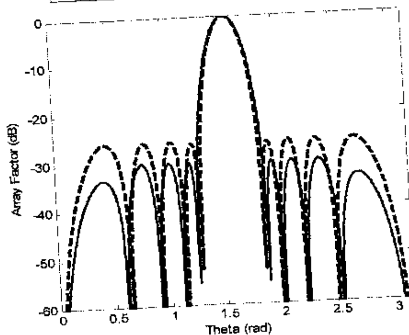
Figure (5): Comparison of patterns of N=10 , d=\lambda/2 linear array with excitations found by GA (solid line) and Dolph-Chebyshev method (dash line)
