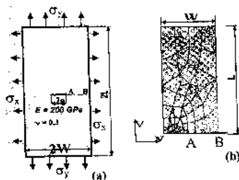
Fig.(8) A plate with central crack under biaxial load
