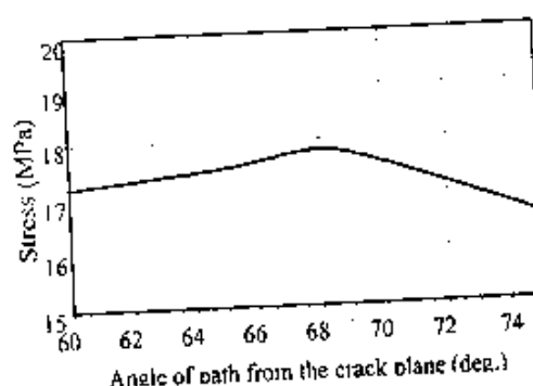
Fig.(16) The angle of maximum \sigma_{yy} around crack tipat r=0.1 w under uniaxial load
