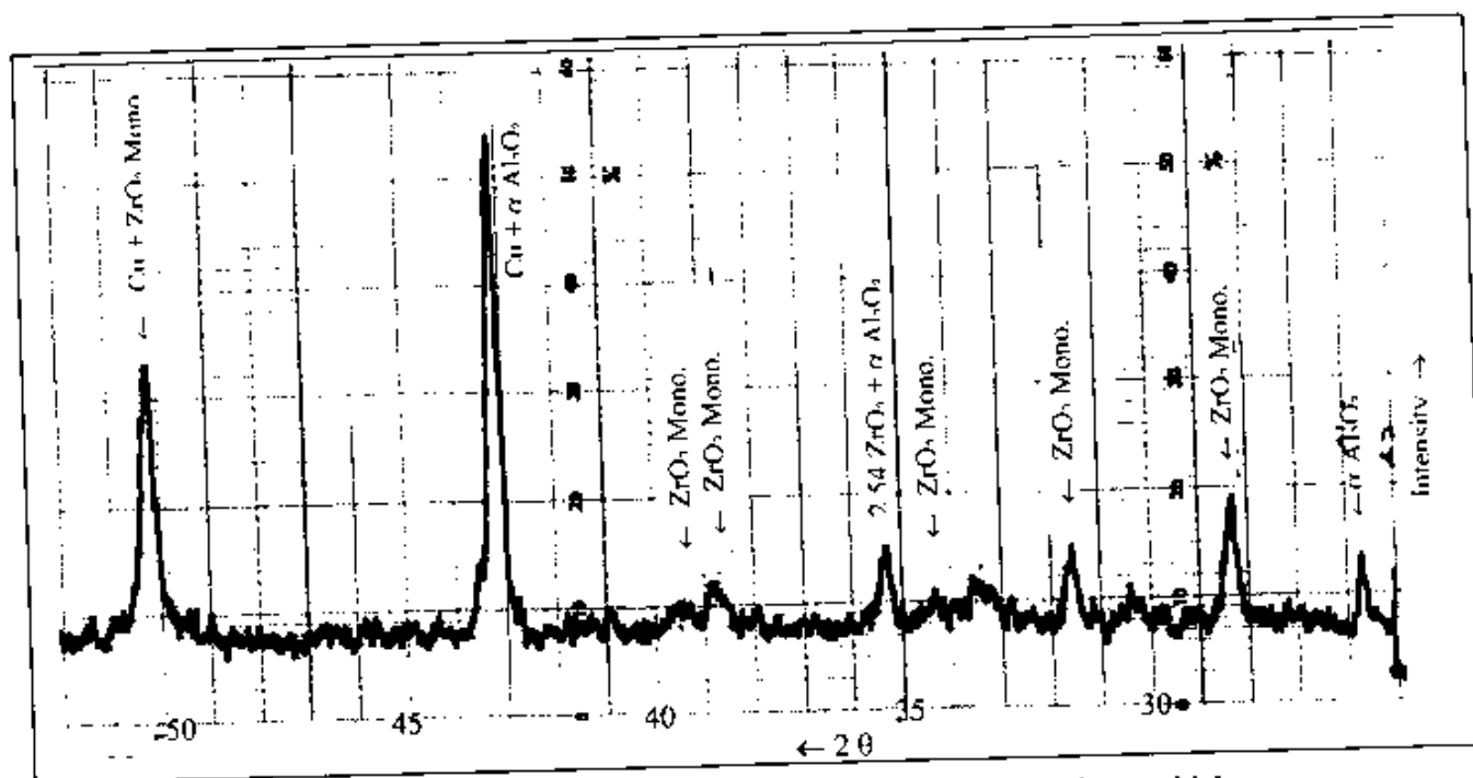
Fig. 11 The XRD pattern of ceramic-to-ceramic fracture surface, which uses CuZr2 as active paste filler-metal, using heating procedure regime No.2
