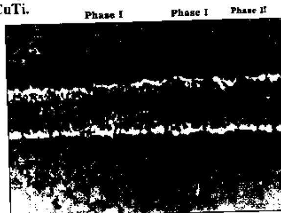
Fig. 9 Bonding line showing ceramic-to-ceramic bonded by active brazing filler-metal alloy type AgCuTi. It shows also two phases, Phase I represents the interfering phase and Phase II represents the matrix phase, X280.
