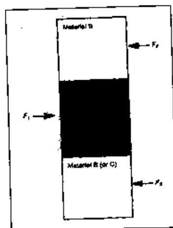
Fig.4 Schematic illustration of the double brazed shear test. [11]
