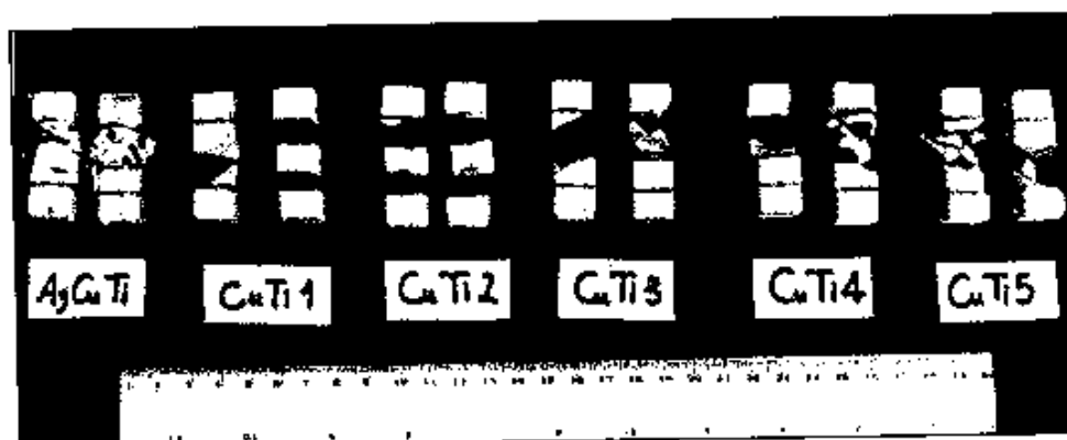
Fig. 15 The DBS fracture pictures for the filler-metal alloys types Cu-Ti and Ag-Cu-Ti systems.
