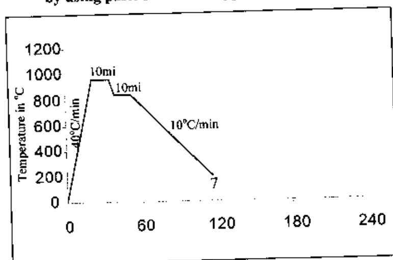
Fig. 7 Heating procedure for double butt joints actively brazed by using paste filler metal type AgCuTi.
