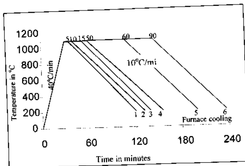
Fig. 6 Heating procedure for double butt joints actively brazed by using paste filler metal type CuTi2.
