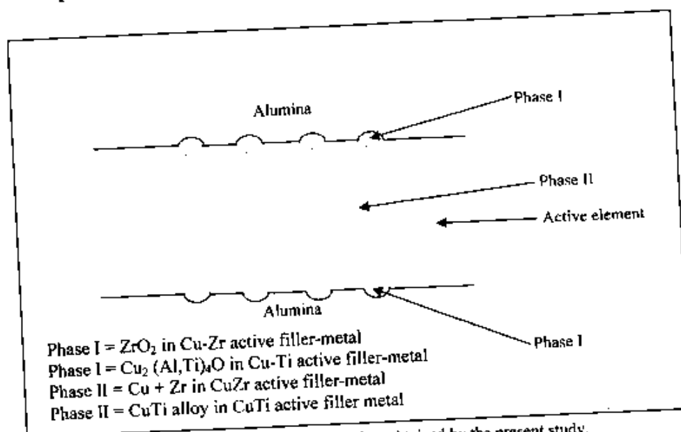
Fig. 13 Suggested bonding mechanism obtained by the present study.
