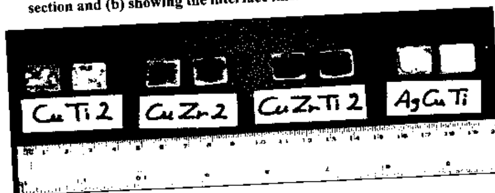
Fig. 3 Photograph shows different types of single-butt joints, using different active filler-metal alloys. CuTi2 and CuZr2 brazed using true filler-metal, while CuZrTi2 and Ag-Cu-Ti were brazed using paste filler-metals.
