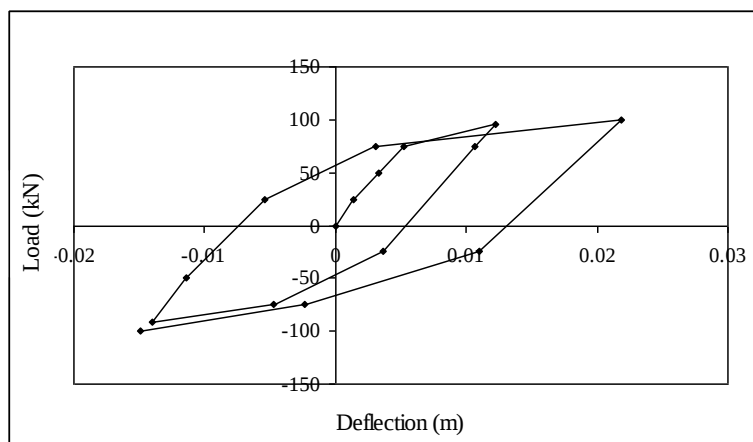
Fig. (9) Load-deflection Relationship of Beam
