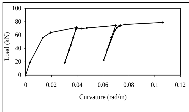
Fig. (12) Moment-curvature relationship of beam P1 under partial repeated loa
