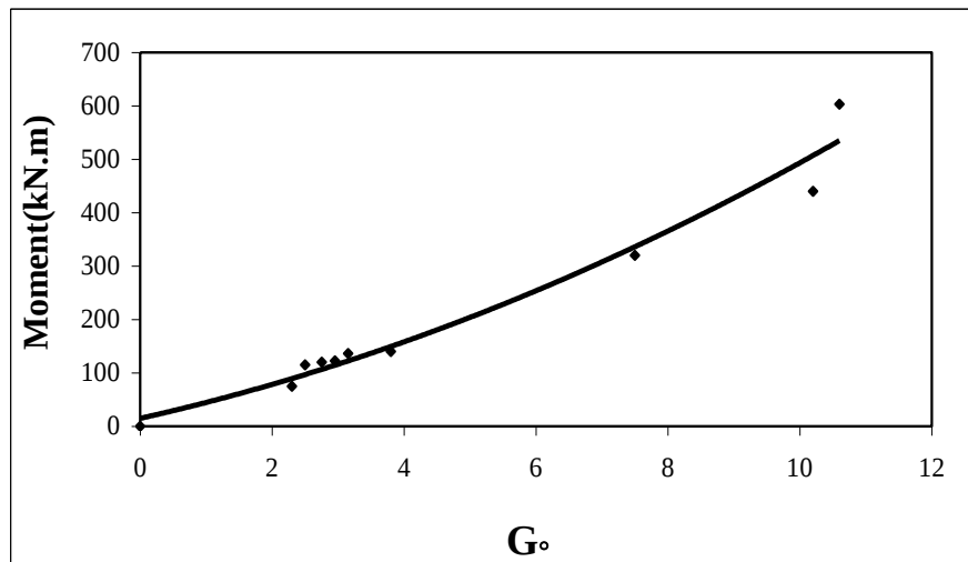
Fig (5) Relation between moment and G_o .
