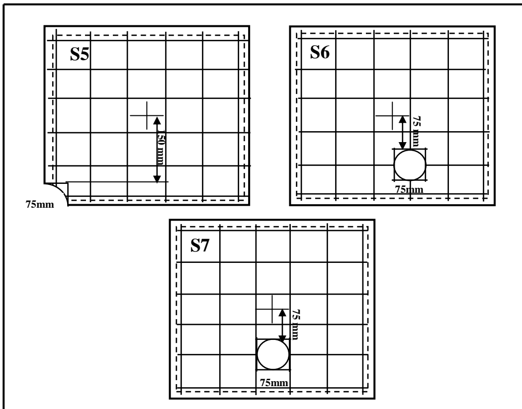
Fig. (4) Dimensions and Reinforcement Details of Slabs in Group (B)
