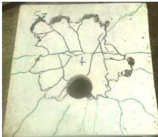
Fig.(21) Crack Pattern at Failure for Specimen S7.
