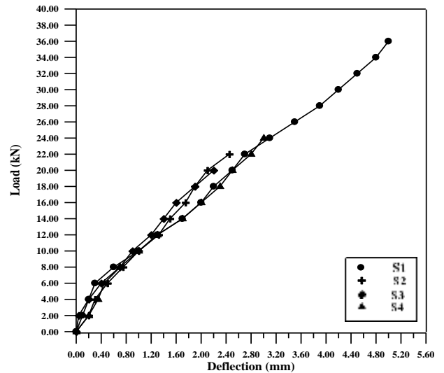
Fig. (13) Load-Deflection Curve of Specimens, S1,S2,S3,S4
