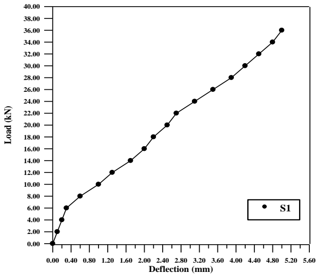
Fig. (6) Load-Deflection Curve of Slab (1)
