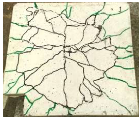
Fig.(18) Crack Pattern at Failure for Specimen S4.
