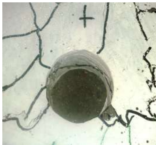
Fig.(23) Crack Pattern at Failure for Specimen S7 within The Opening.
