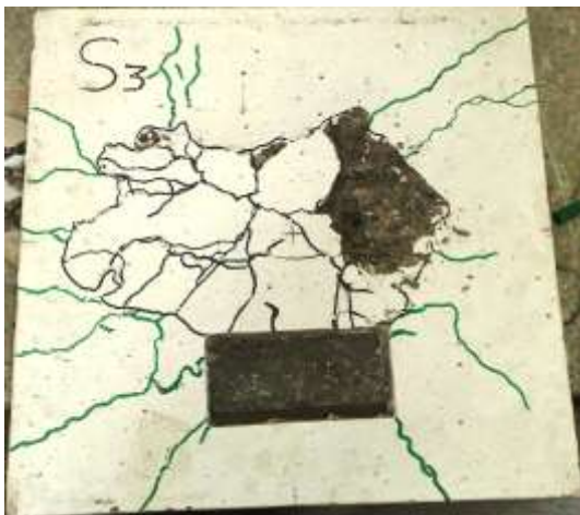
Fig.(17) Crack Pattern at Failure for Specimen S3.
