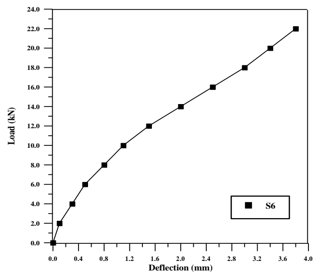
Fig. (11) Load-Deflection Curve of Slab (6)
