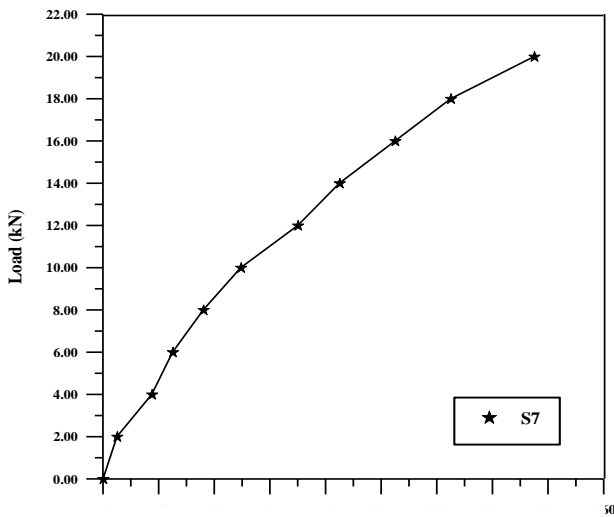
Fig. (12) Load-Deflection Curve of Slab (7)
