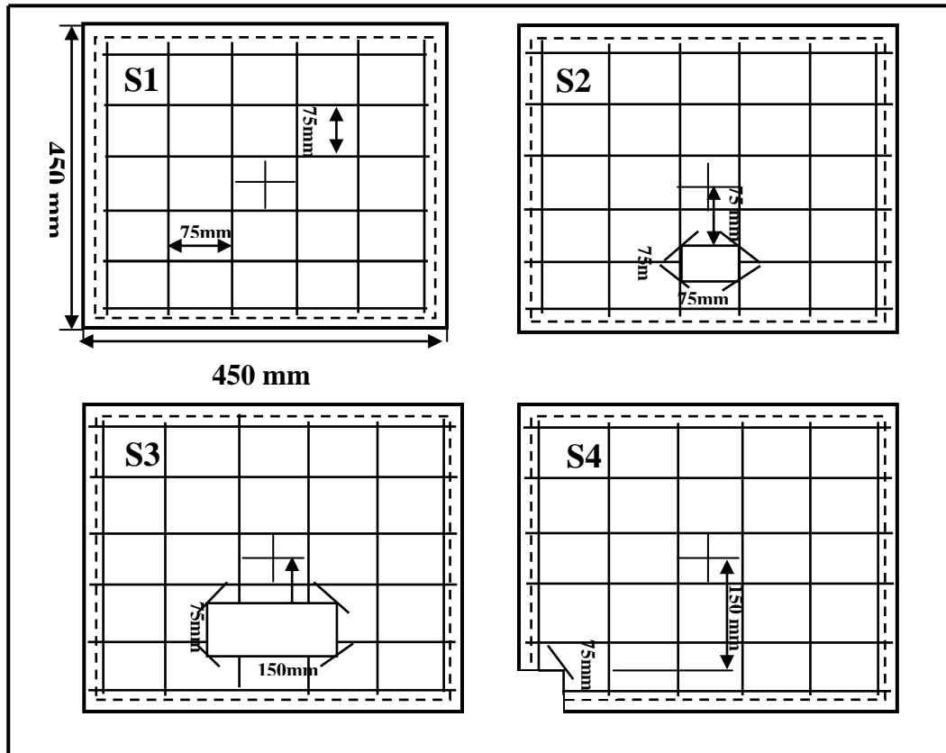
Fig. (3) Dimensions and Reinforcement Details of Slabs in Group (A)
