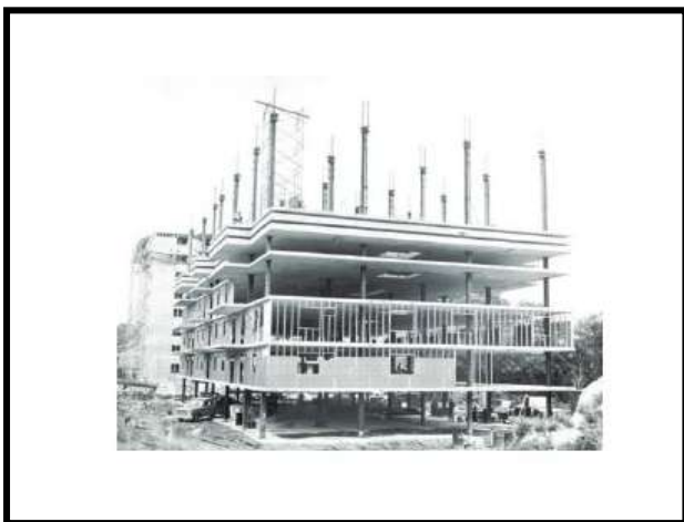
Fig. (1) Lift Slab System (2)
