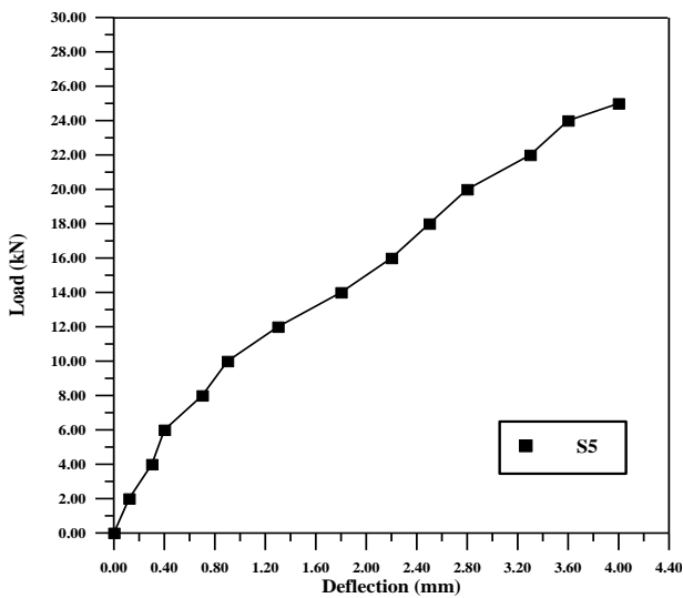
Fig. (10) Load-Deflection Curve of Slab (5)
