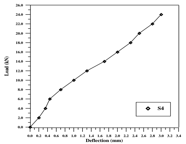
Fig. (9) Load-Deflection Curve of Slab (4)
