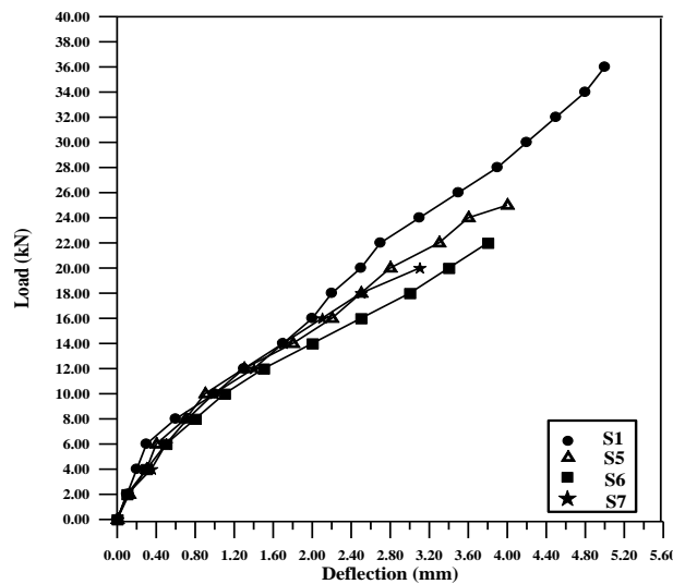
Fig. (14) Load-Deflection Curve of Specimens, S1, S5, S6, S7
