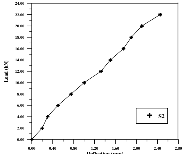
Fig. (7) Load-Deflection Curve of Slab (2)
