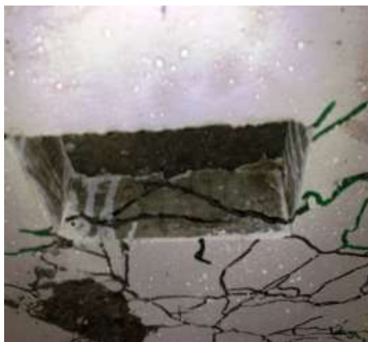
Fig.(22) Crack Pattern at Failure for Specimen S3 within The Opening.
