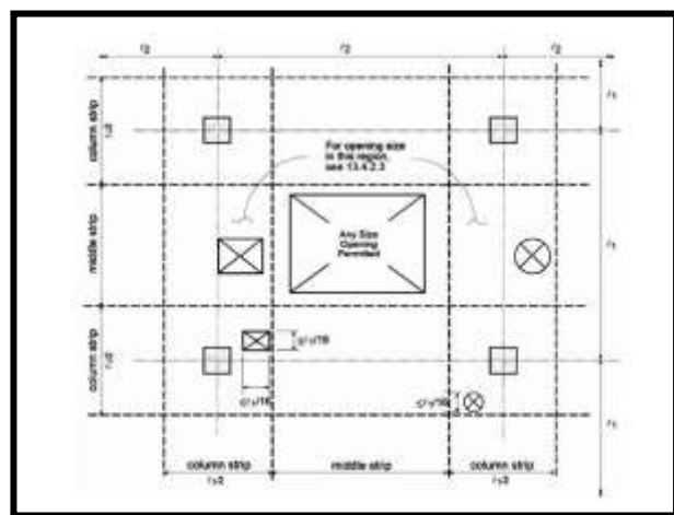
Fig. (2) Suggested Opening Sizes and Locations in Flat Slabs (4)
