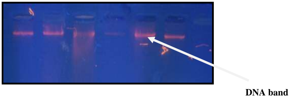
Figure 1- Bands of total DNA on 1% agarose gel , one hour electrophoresis .
