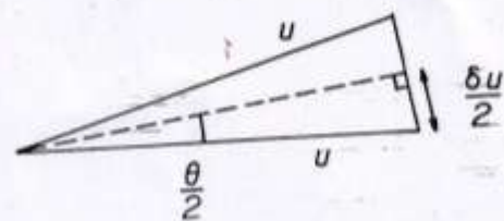
Fig. 5. Vector diagram relating \delta\vec{u} to \vec{u} and \theta .
