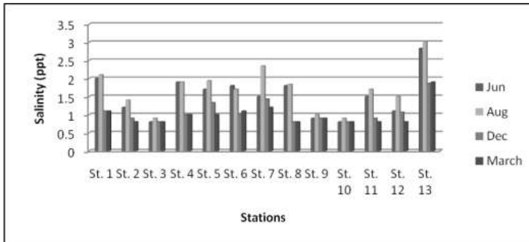
Fig. 4 the salinity concentration during period of study (ppt) in Al-Hwaizeh marsh.
