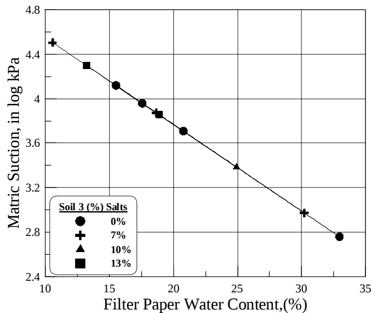
Figure (16) Relationship between the matric suction and filter paper water content for soil 3 mixed with different percentages of salt.
