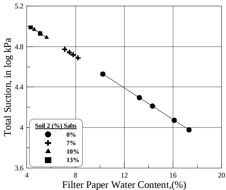
Figure (12) Relationship between the total suction and filter paper water content for soil 2 mixed with different percentages of salt.
